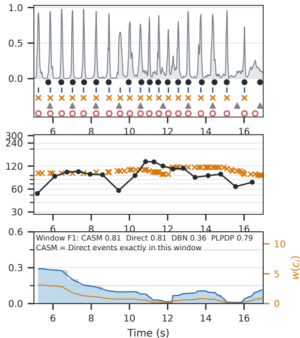
(b) Ambiguous evidence: CASM defers Beat This / SMC OOF · smc/smc_043
