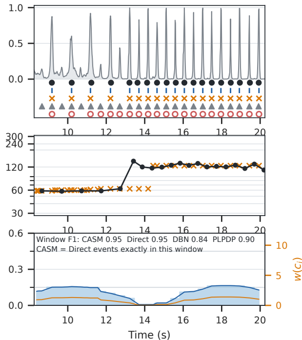
(b) Ambiguous evidence: CASM defers Beat This / SMC OOF · smc/smc_032
