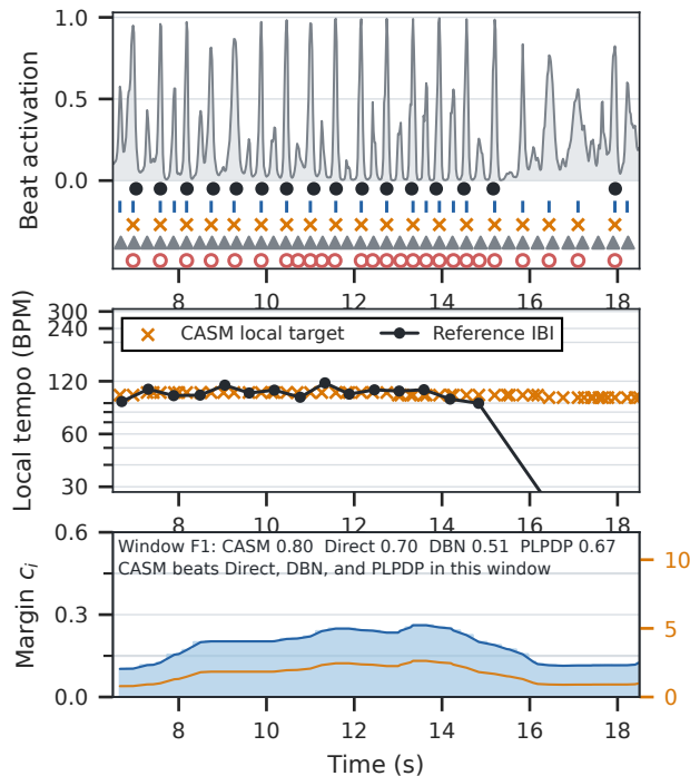
(a) Clear periodicity: CASM wins across decoders Beat This / SMC OOF · smc/smc_098
