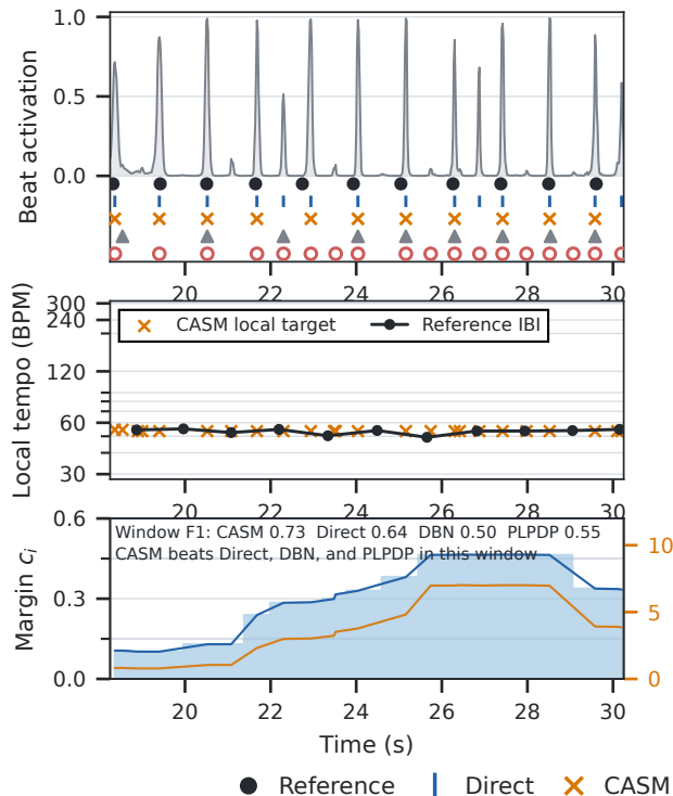
(a) Clear periodicity: CASM wins across decoders Beat This / SMC OOF · smc/smc_221
