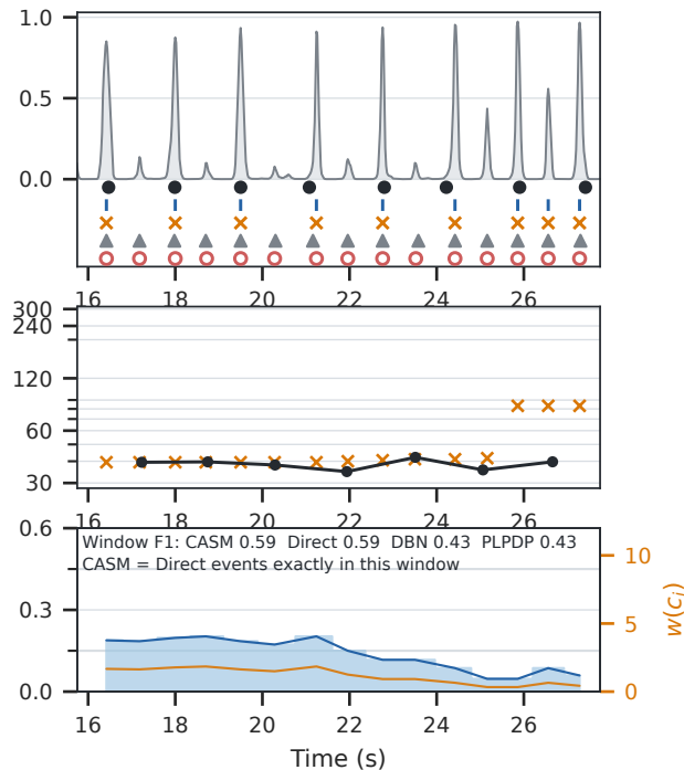
(b) Ambiguous evidence: CASM defers Beat This / SMC OOF · smc/smc_005
