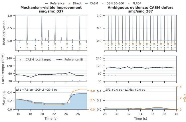
Fig. 1. Two held-out SMC excerpts illustrating CASM on Beat This activations. A well-separated local period recovers weak, activation-supported beats (left); competing periods relax the duration constraint, producing the Direct path in this example (right). Reference beats and IBI are shown only for interpretation and are not decoder inputs.
