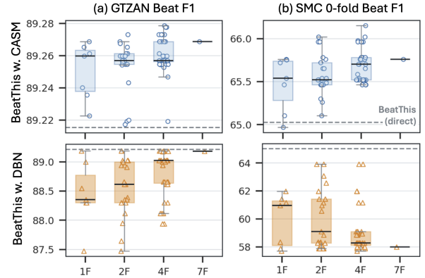
Fig. 2. Here is explain how to train Semi-Markov... about the data scaling problem
