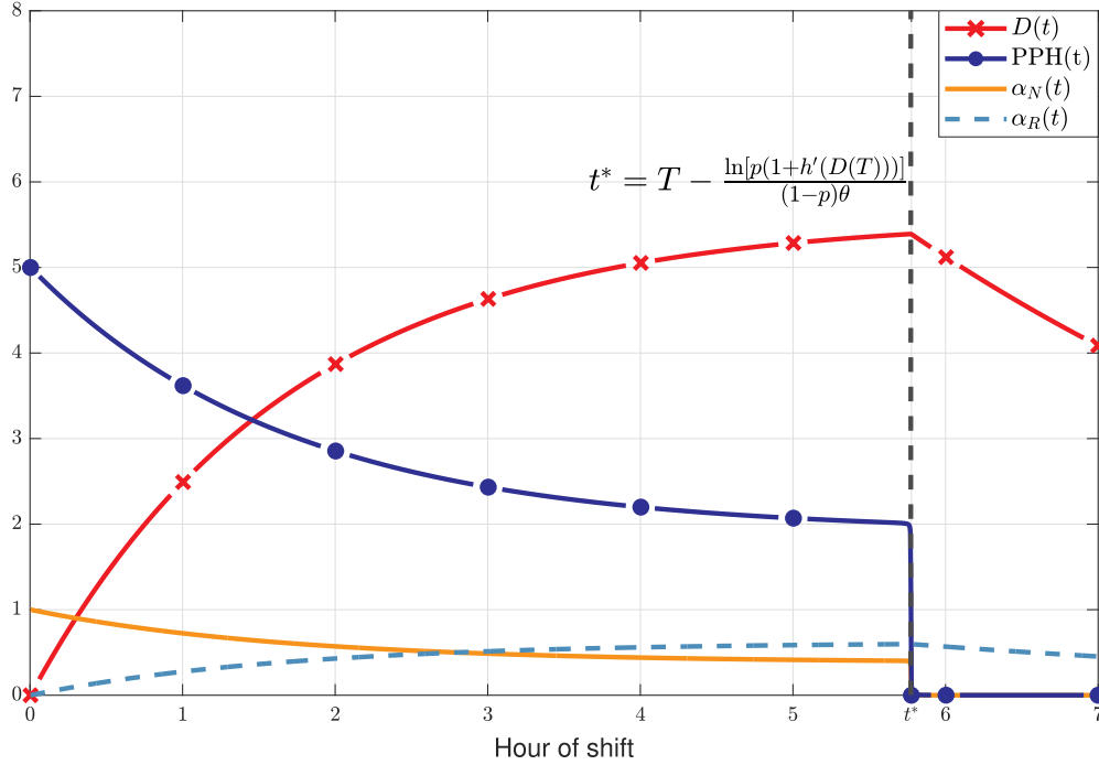
Figure 6. (Color online) Numerical Illustration of \alpha_N^*(t) , \alpha_R^*(t) , D(t) , and PPH(t) Under the Optimal Policy for Problem (2) When D_0 = 0, R_0 = 0, \mu_N = 5, \mu_R = 6, \theta = 0.6, p = 0.66, h(x) = x , and T = 7 (i.e., Seven-Hour Shifts)
