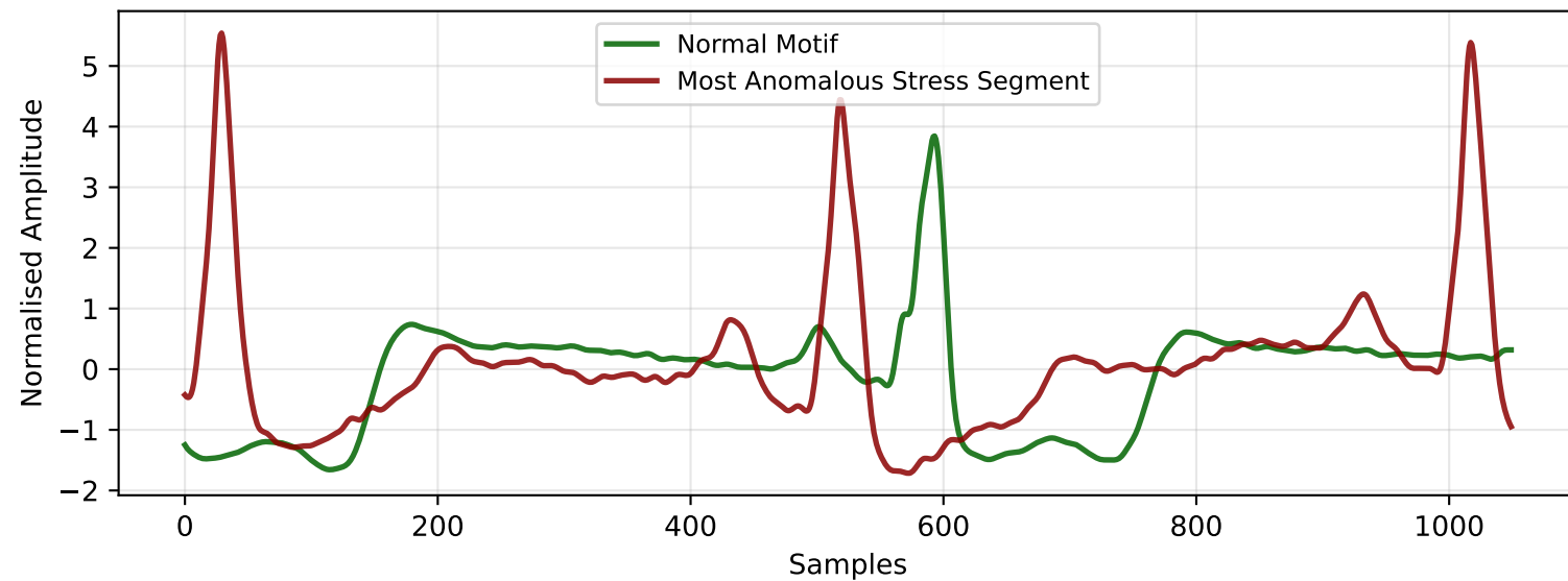
S2 : Motif vs. Most Anomalous Segment Distance = 43.391 (motif mean = 41.032)
