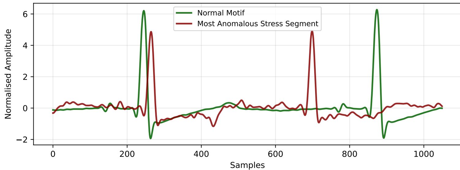
S8 : Motif vs. Most Anomalous Segment Distance = 46.180 (motif mean = 43.694)
