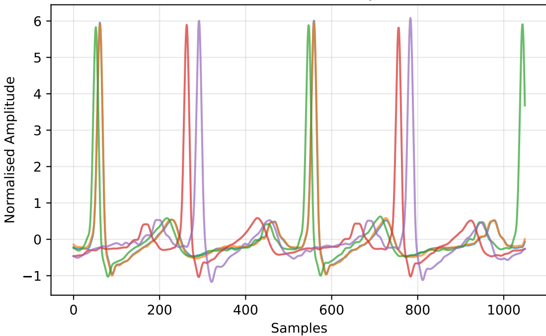
S13 — All 5 Motifs Comparison
