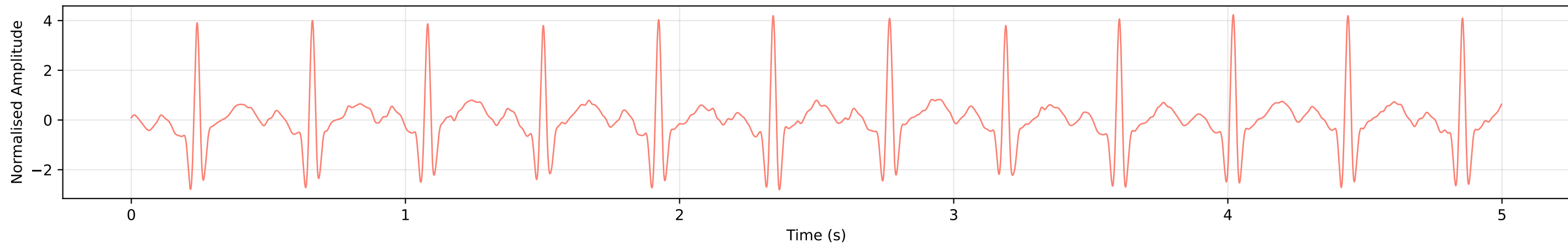
S14 — Cleaned Stress ECG
