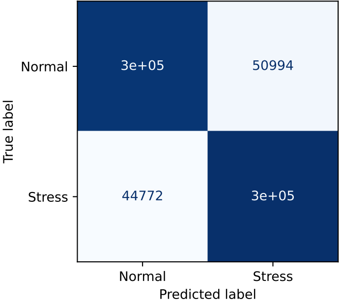
Confusion Matrix
