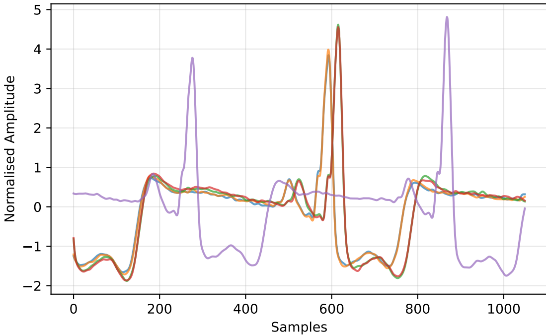
S2 — All 5 Motifs Comparison
