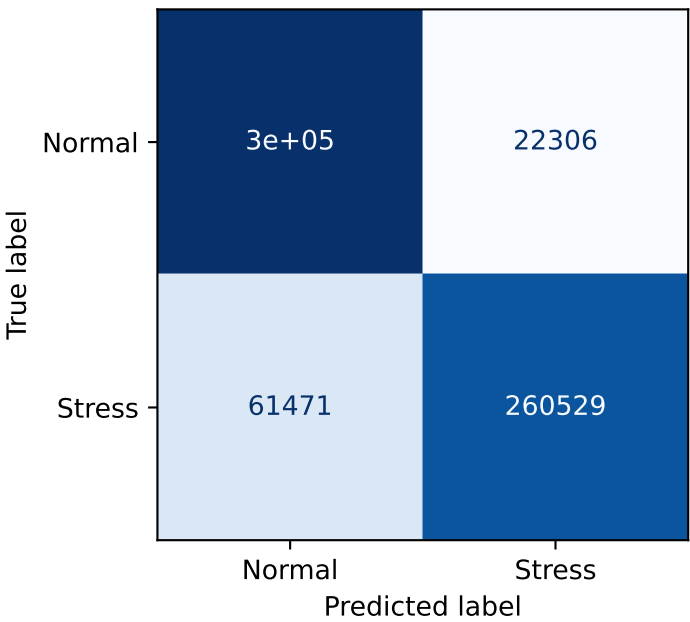
Confusion Matrix
