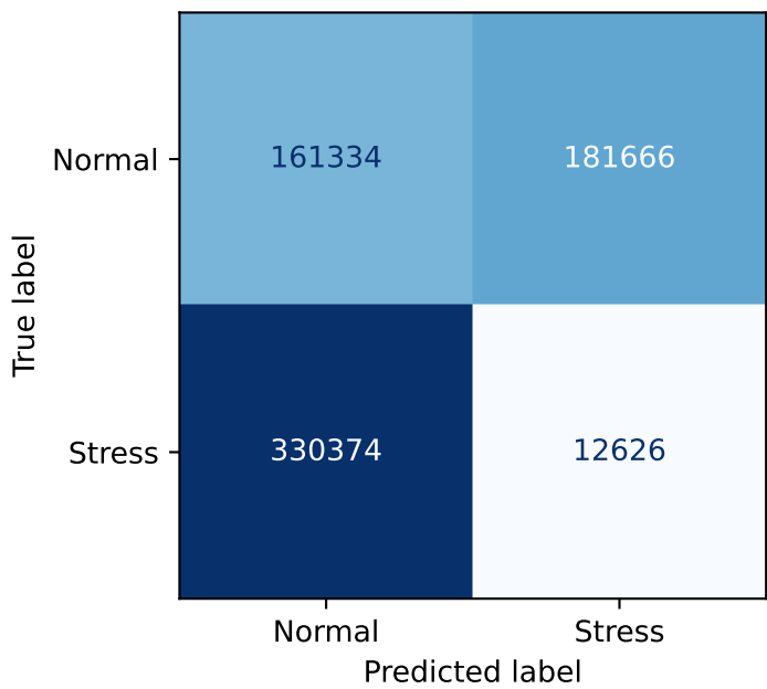
Confusion Matrix
