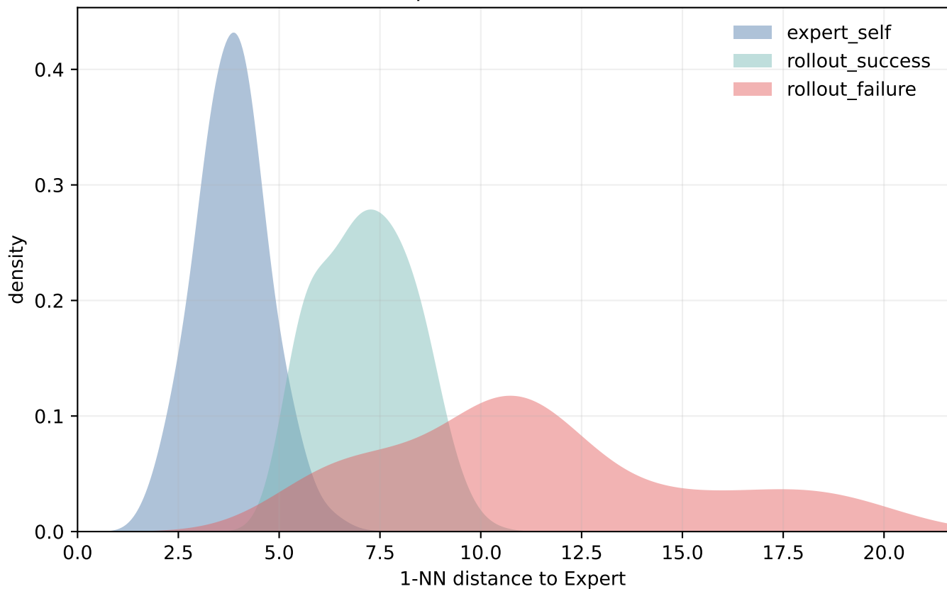
L2-Visual: 1NN to expert · frame-level (all frames, linear)
