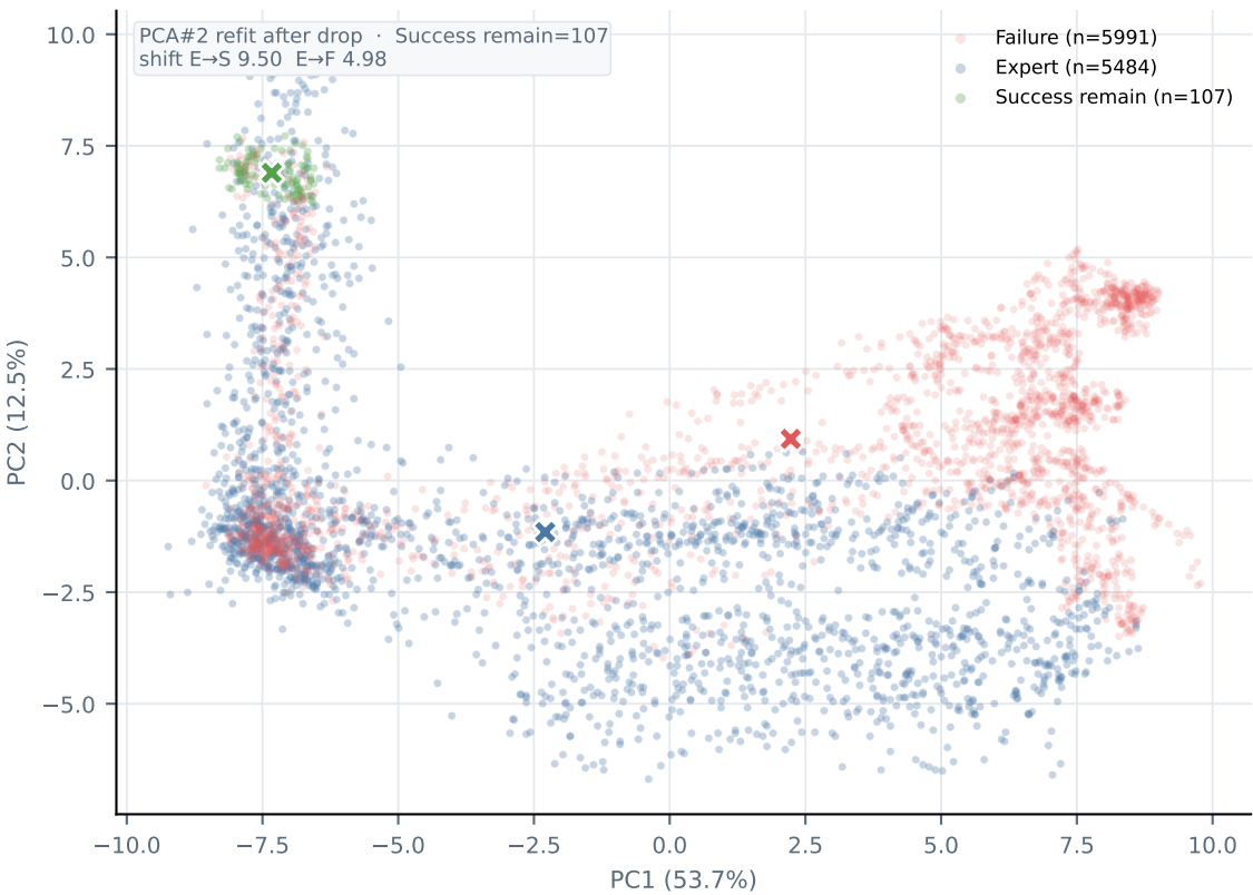
② PCA#2 scatter · after drop + refit
