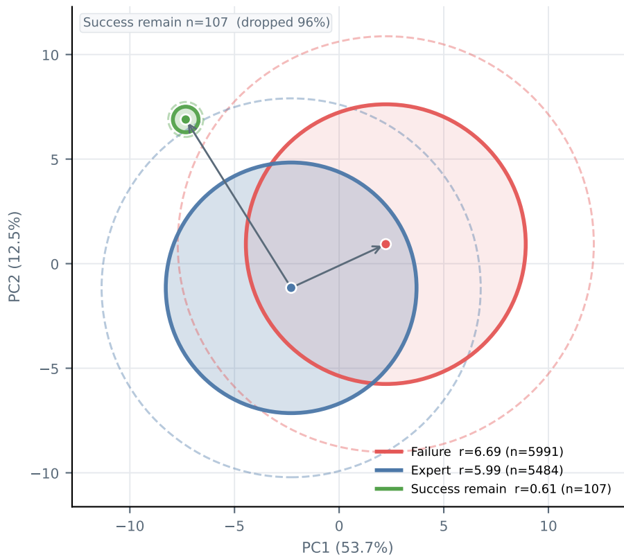
② PCA#2 circles · after drop + refit
