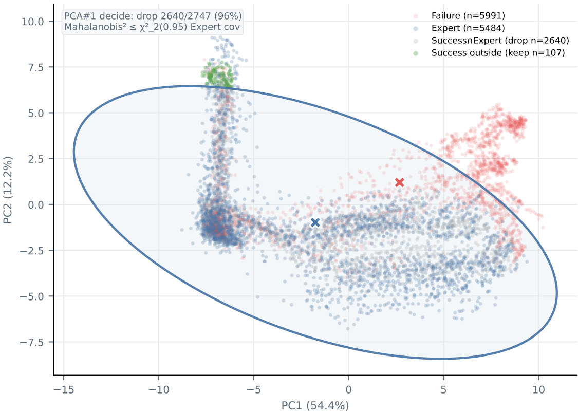
① PCA#1 scatter · decide membership
