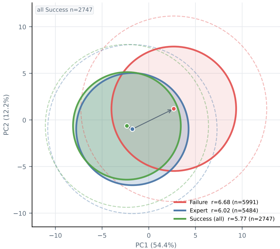
① PCA#1 circles · before drop
