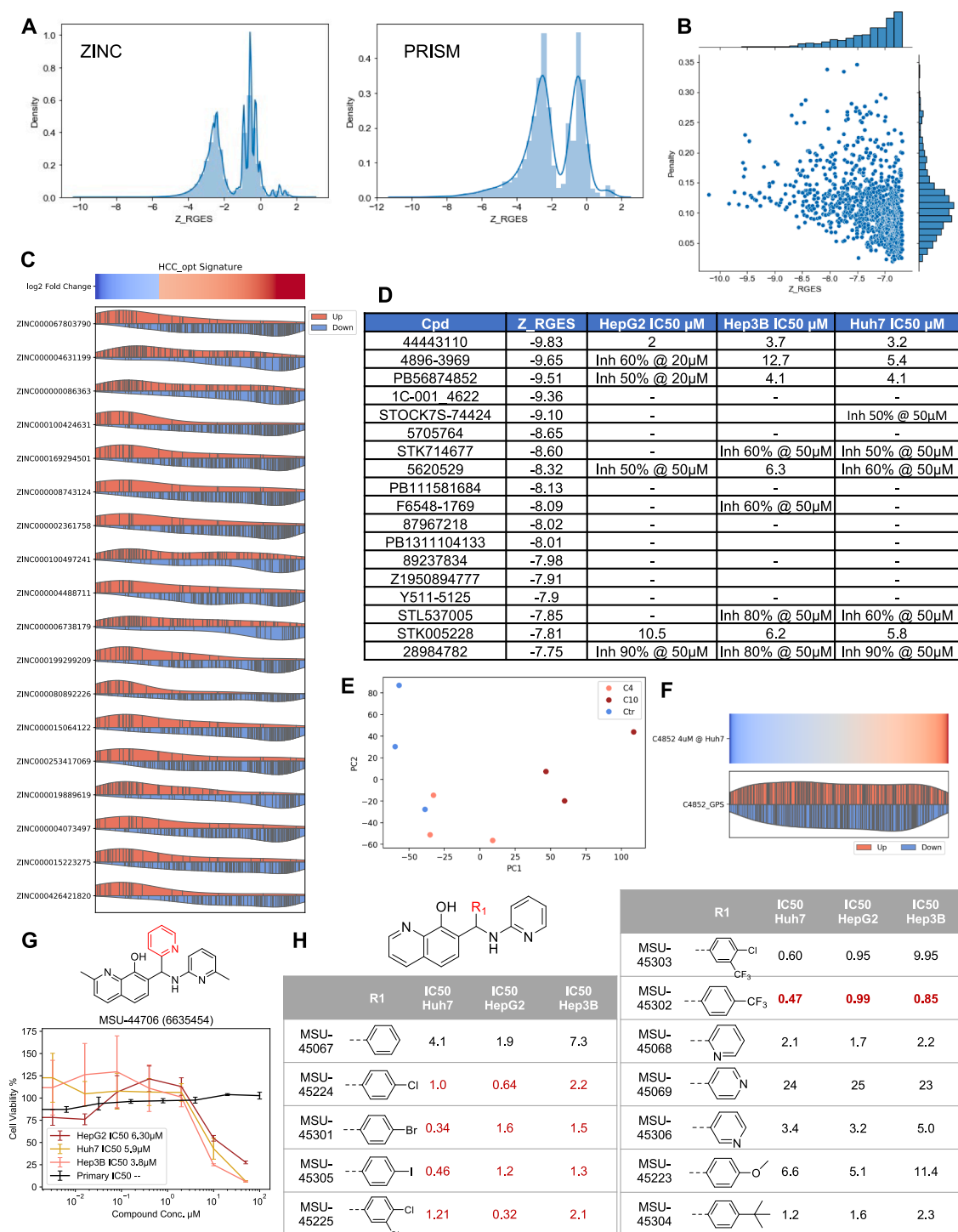
Figure S4. The virtual screening and identification of anti-HCC hits from millions of compound profiles generated by GPS, related to Figure 4
