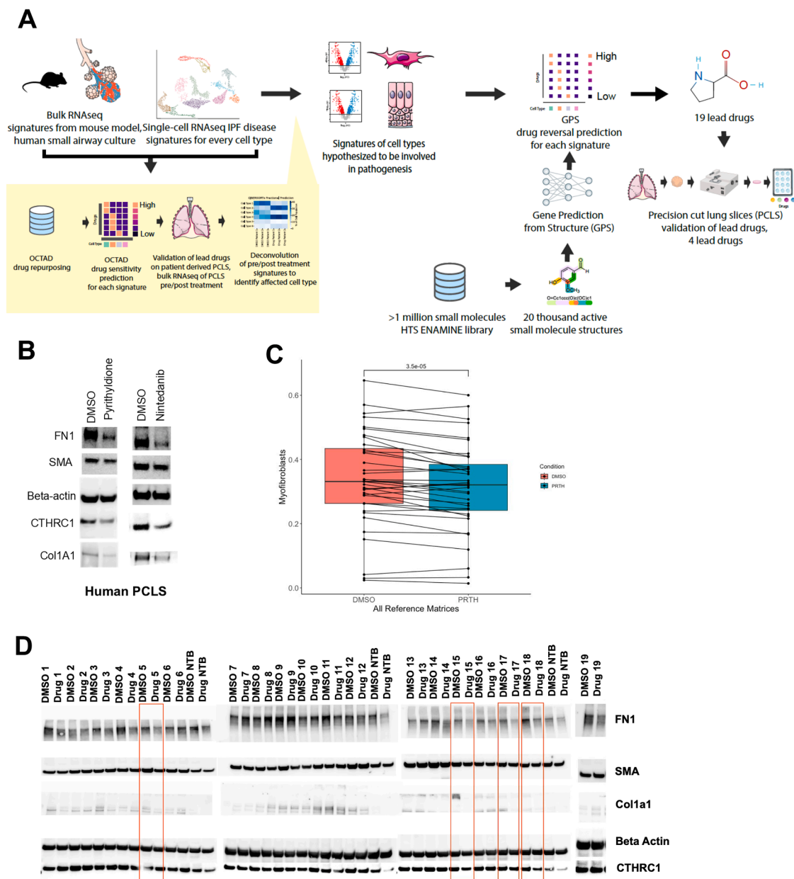
Figure S6. Drug discovery against IPF using GPS, related to Figure 6
