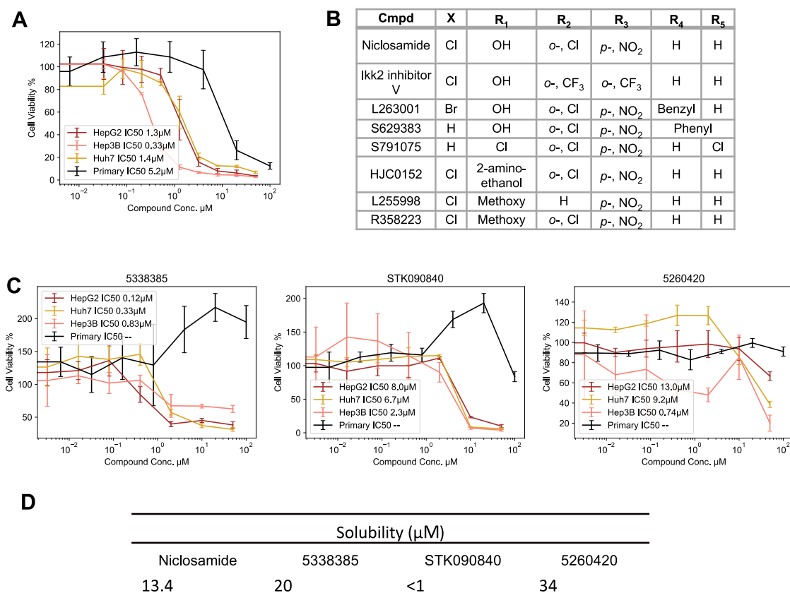
Figure S3. Validation of reversing the HCC signature using GPS-predicted compound profiles, related to Figure 3
