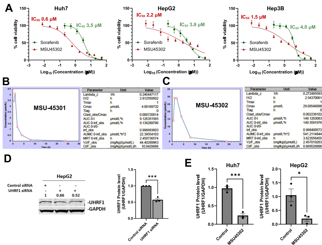
Figure S5. Hit-to-lead optimization of the anti-HCC candidate, related to Figure 5
