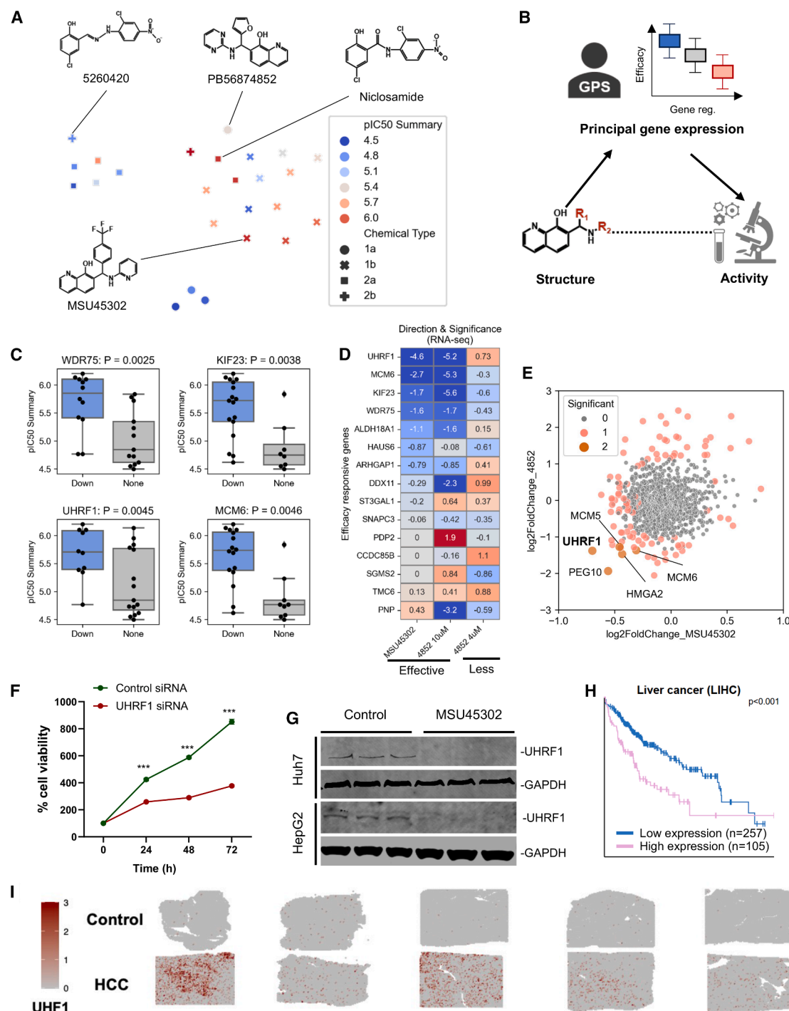
Figure 5. SGAR for HCC drug discovery and MoA interpretation
