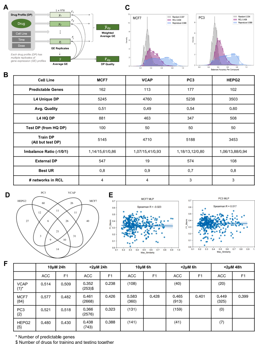
Figure S1. Details of GPS data, performance, and application summary, related to Figure 1
