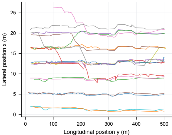
Representative cleaned NGSIM tracks
