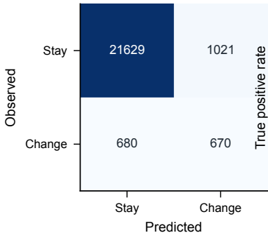
Confusion matrix
