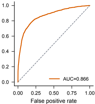
ROC curve
