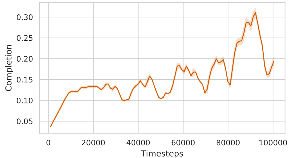
Shaped Reward
