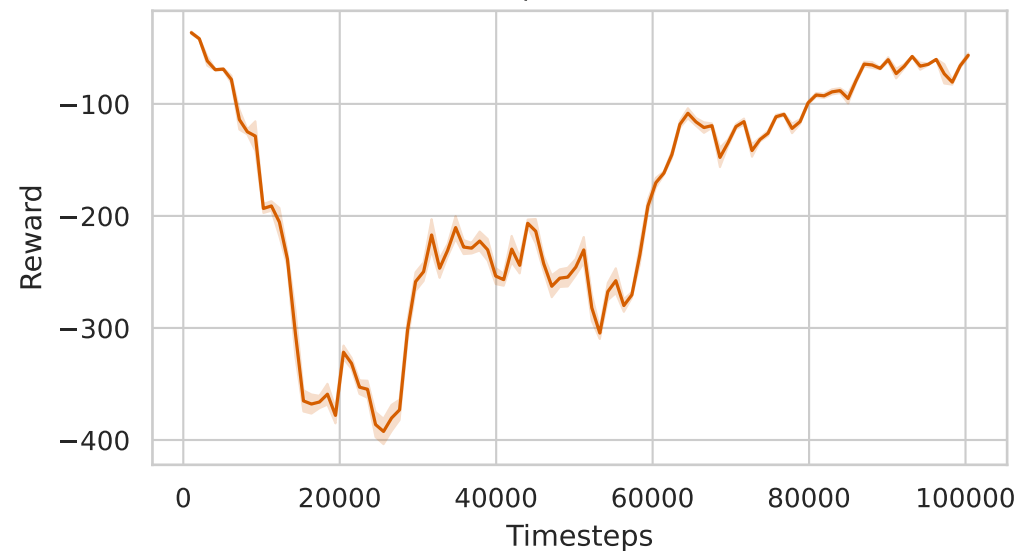
Shaped Reward
