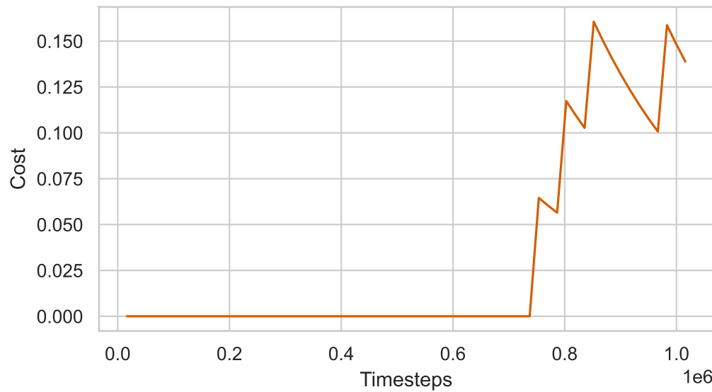
Safety Cost
