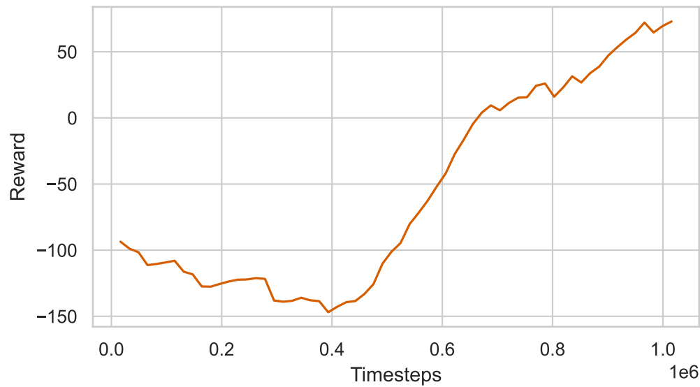
Shaped Reward
