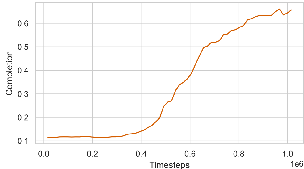
Shaped Reward
