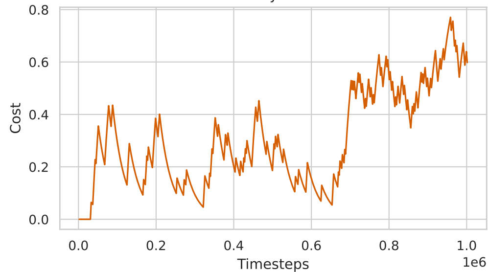
Safety Cost
