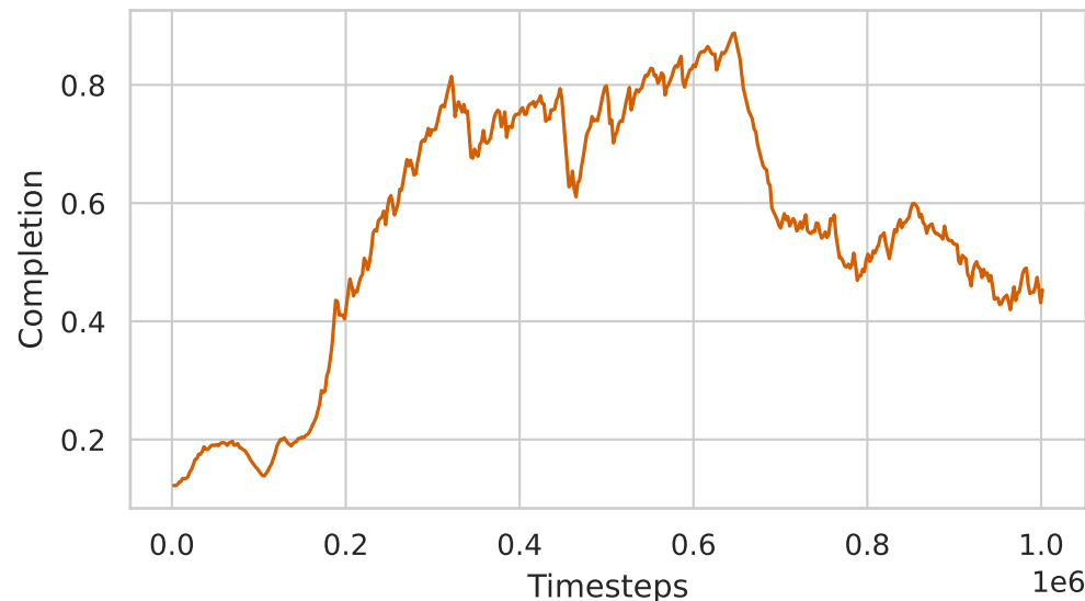
Shaped Reward
