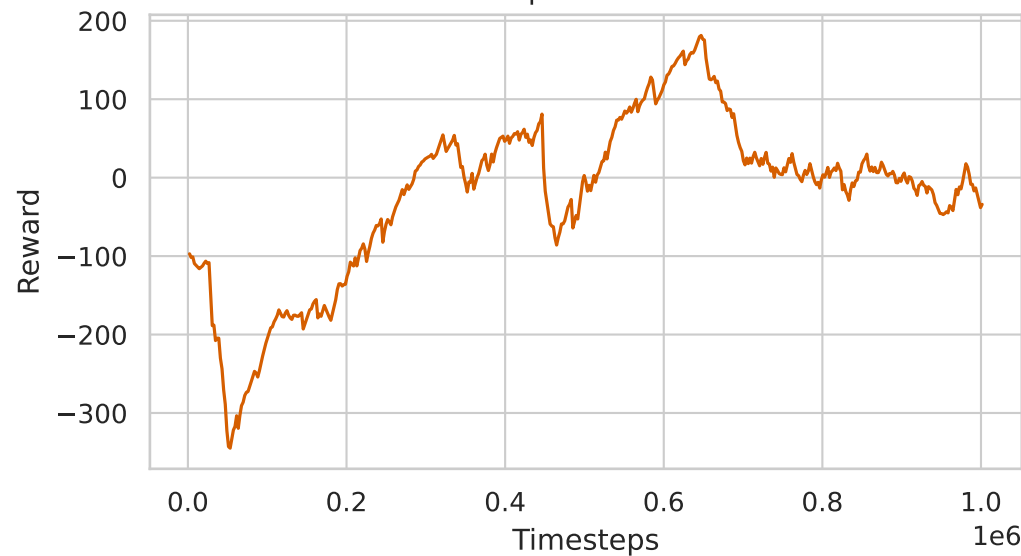
Shaped Reward
