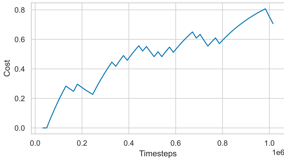
Safety Cost
