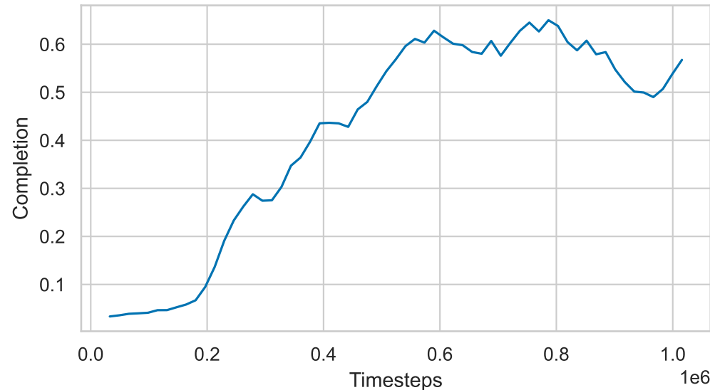
Shaped Reward
