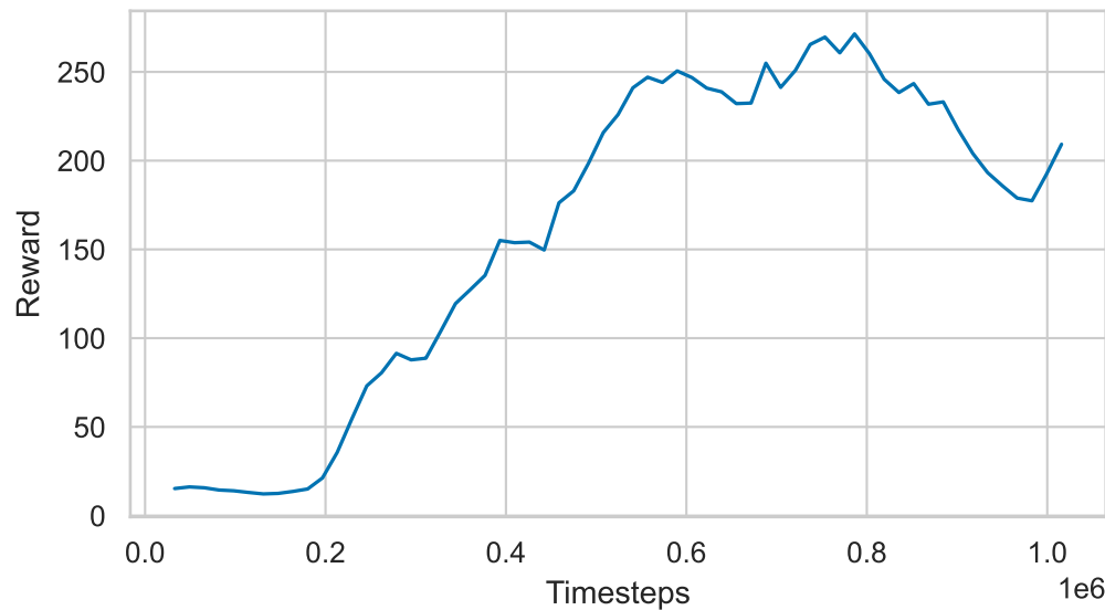
Shaped Reward
