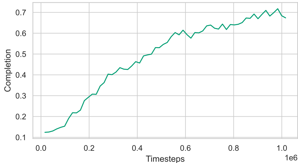
Shaped Reward
