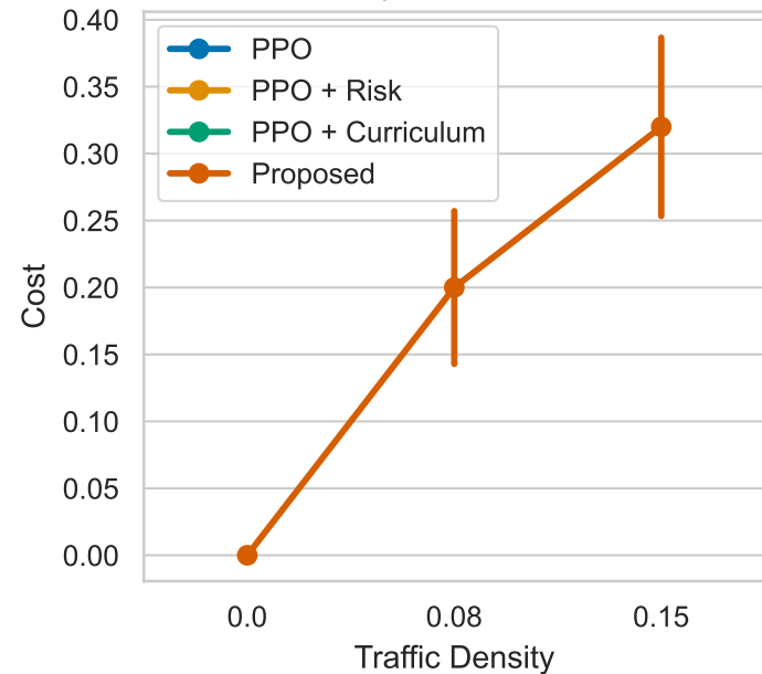
Episode Cost
