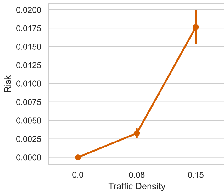
TTC Risk
