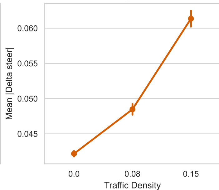
Steering Variation
