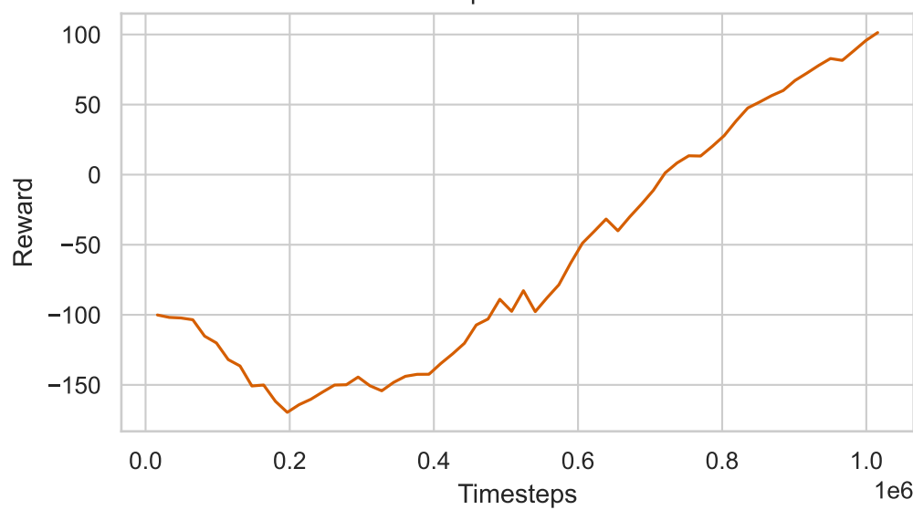
Shaped Reward
