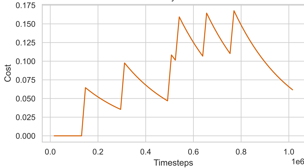
Safety Cost
