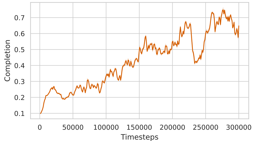
Shaped Reward
