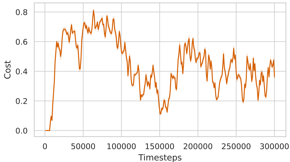
Safety Cost
