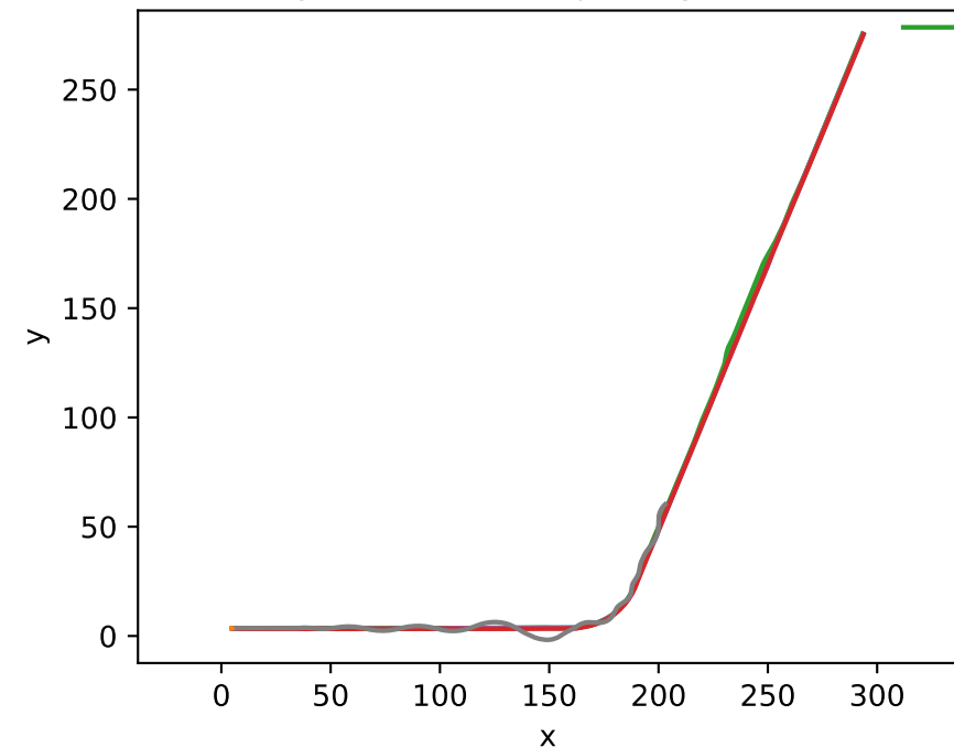
Representative trajectory d=0.15
