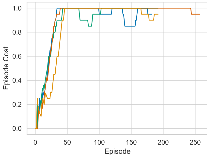
Training Safety Cost (Rolling Window)
