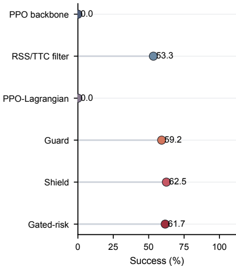
External comparison
