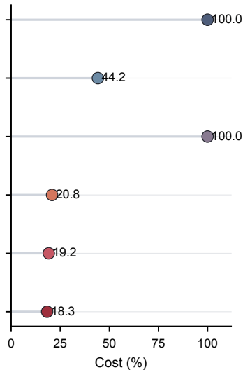
PPO-Lagrangian baseline
