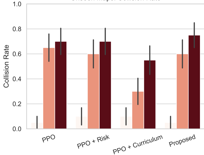
Unseen Maps: Collision Rate
