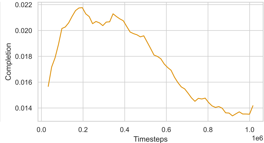
Shaped Reward
