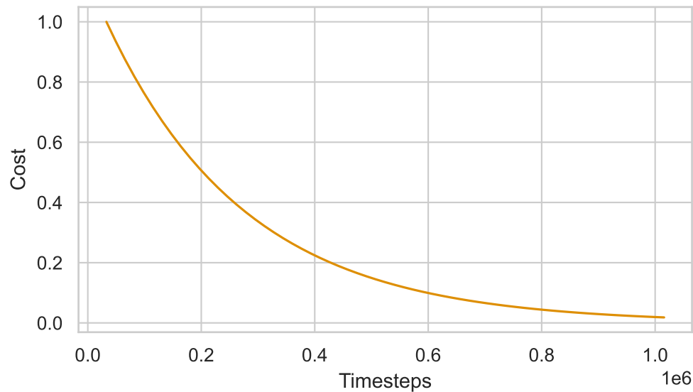
Safety Cost
