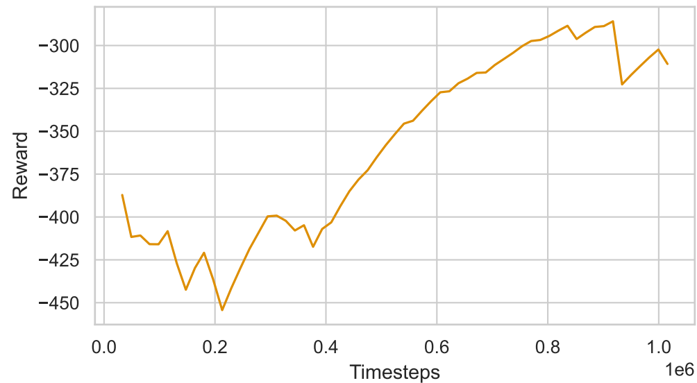
Shaped Reward
