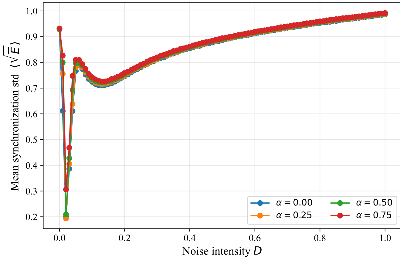
Mean sync-std vs D at fixed \tau = 0.10
