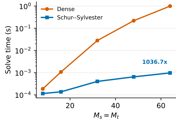
(a) Structured solver scaling
