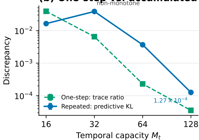
(b) One-step vs. accumulated discrepancy
