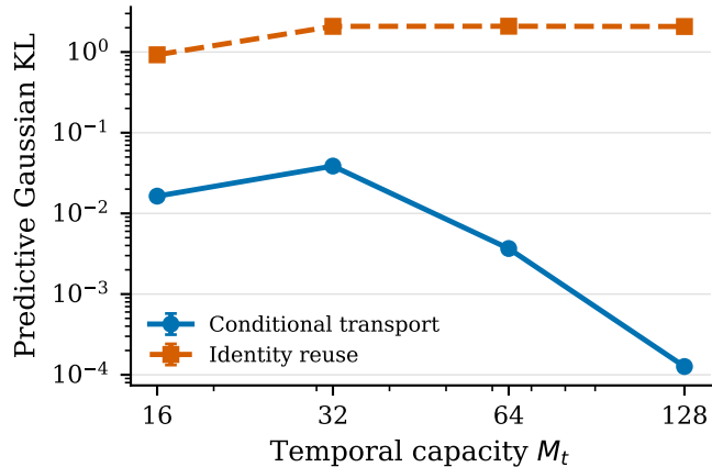
(b) Predictive KL
