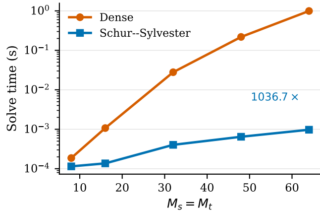
(c) Solver scaling
