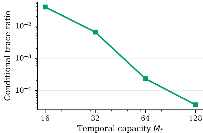
(a) One-step projection discrepancy
