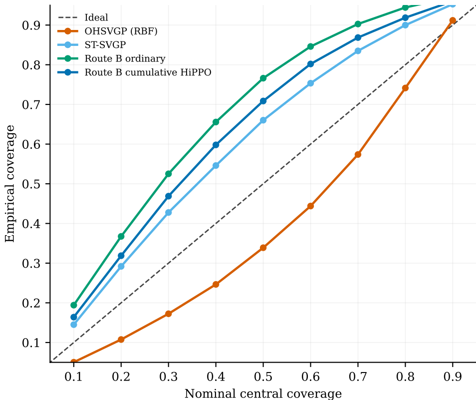
Gaussian predictive calibration
