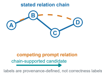
c Controlled relation-graph assay
