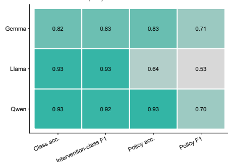
Fig. 5 | A bounded local actuator controls trajectories and a declared output boundary. a, Additive failures, bounded actuator and gate. b, Real-versus-fixed internal specificity. c, Real policy versus 50 joint-label shuffles. d, Classifier quality. e, Strict full-vocabulary conflict-to-clean crossings among 87 held-out closure prompts and collateral changes among 203 non-closure prompts: Qwen, 17/87 and 0/203; Llama, 13/87 and 2/203; Gemma, 9/87 and 0/203. Clean is provenance-defined; counts do not measure accuracy. See Extended Data Fig. 6f for action reassignment, Supplementary Methods Table 5 for non-crossings, and Source Data Fig. 5 and manifest.
