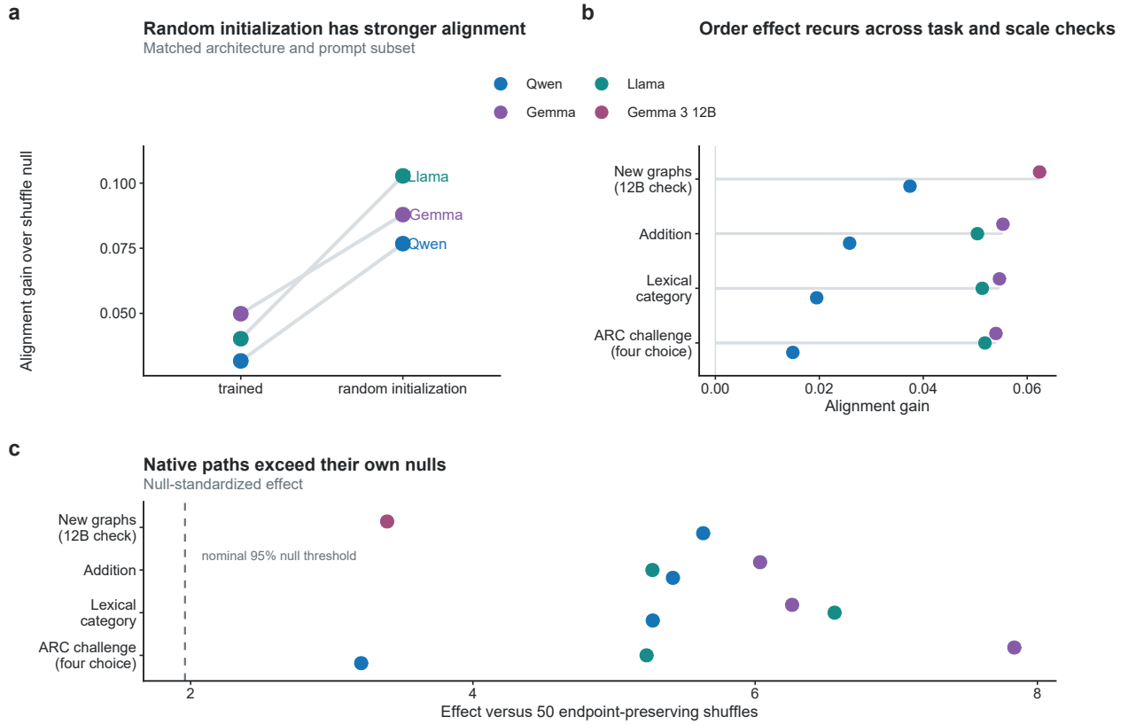
Fig. 2 | Architecture-compatible propagation scaffold. a, Random initializations show larger alignment gains than their trained checkpoint counterparts for the tested architectures. b, The native-order alignment contrast recurs across controlled addition, lexical and ARC-Challenge audits and in a paired 12B new-graph confirmation. c, Every displayed task-model pair exceeds its 50 endpoint-preserving shuffles on its own null-standardized scale. The 12B result is a checkpoint-specific confirmation, not a pure scale law because family, quantization and capture runtime differ. Strong alignment alone is not evidence of learned reasoning. All finite-path metrics are defined against the stated endpoint-preserving null. See Source Data Fig. 2 and the Source Data manifest.
