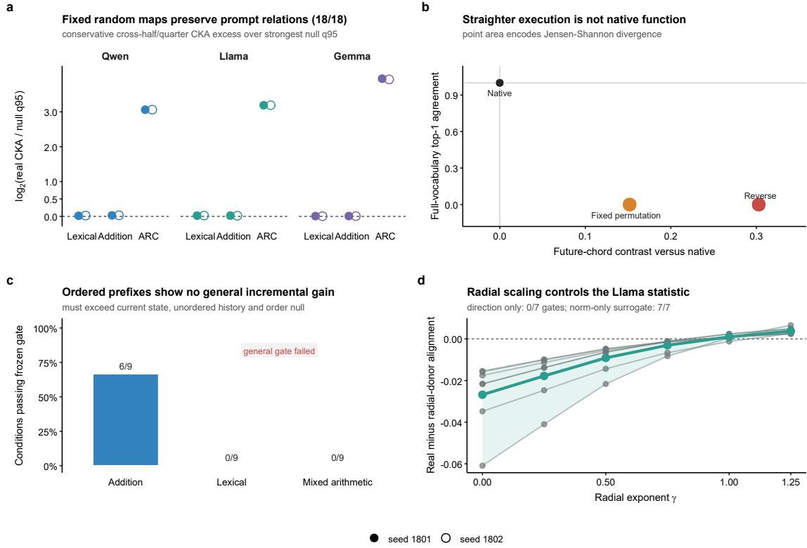
Fig. 18: Falsification controls bound the interpretation of layer-order geometry. a , Random fixed-map relational-continuity contrasts across three architecture configurations, three task families and two seeds; all 18 declared conditions pass the positive-contrast gate. b , Reversed and fixed-permutation Qwen executions retain positive geometry but lose native full-vocabulary outputs. c , Ordered-prefix summaries add held-out signal beyond current state only in 6/9 addition conditions and in neither lexical nor mixed-arithmetic tests. d , Llama chord metrics vary monotonically under frozen radial rescaling. These controls separate architecture-compatible propagation, native ordered execution and metric sensitivity.
