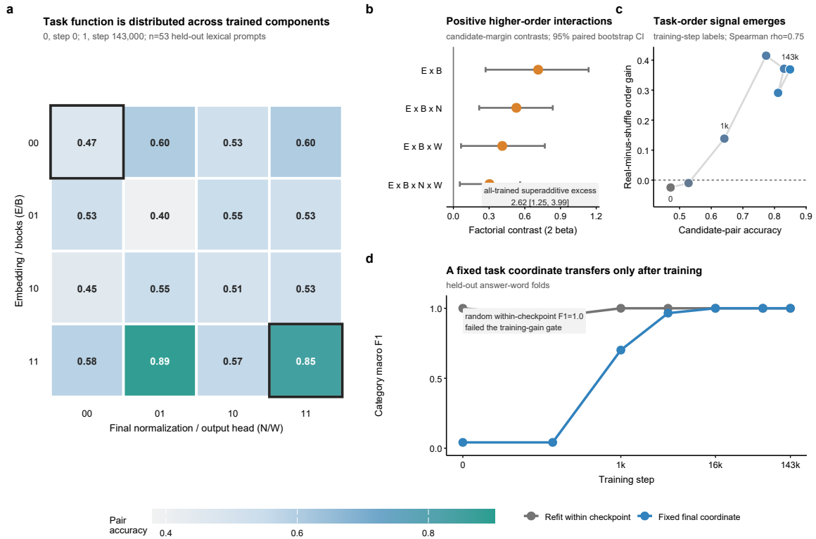
Fig. 19: Training organizes compatible components and task coordinates. a , Accuracy for all initialized/trained combinations of embeddings, blocks, final normalization and output head. b , Higher-order interaction terms; the fully trained system has a positive superadditive margin beyond additive component gains. c , Model-native candidate-coordinate order signal emerges during Pythia training and tracks held-out accuracy. d , A coordinate fixed at the final checkpoint transfers poorly at initialization and becomes predictive during training, whereas within-checkpoint category separation is already perfect at initialization and is therefore a negative control rather than evidence of learning.
