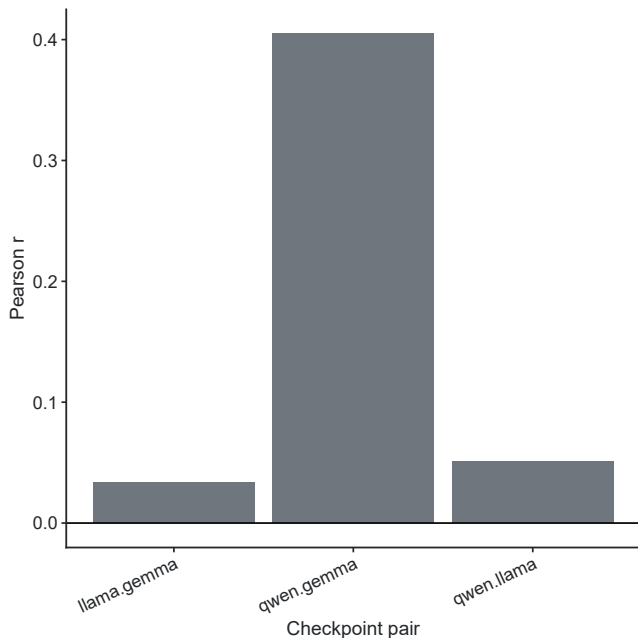
a Direction identity is weak across checkpoints
