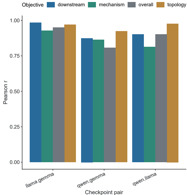
b Functional geometry recurrence depends on objective
