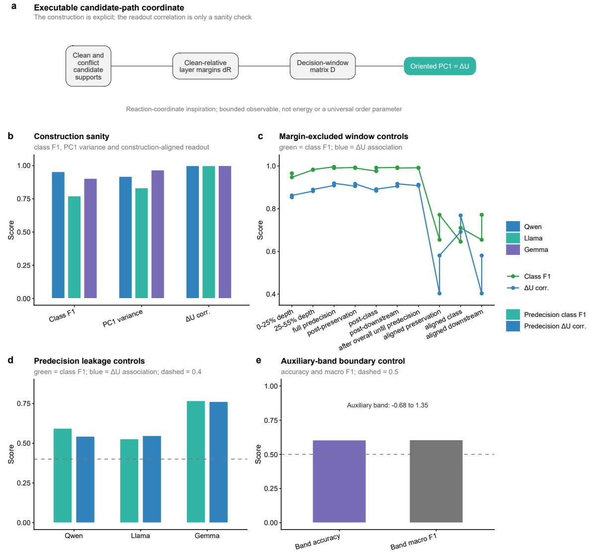
Fig. 3 | Construction and bounds of candidate-path separation. a, Candidate supports define clean- relative layer margins dR , the decision-window matrix D and oriented PC1 score \Delta U . b, Prompt-class F1, PC1 variance and the construction-aligned \Delta U -dominance check. c,d, Candidate-margin-excluded and predecision controls; green is class F1, blue is \Delta U association, and higher values indicate greater retention of the original diagnostic. e, Auxiliary-band accuracy and macro F1. Dashed lines mark 0.4 in d and 0.5 in e. \Delta U is a bounded candidate-path separation observable, not an energy or universal order parameter. See Source Data Fig. 3 and Source Data manifest.
