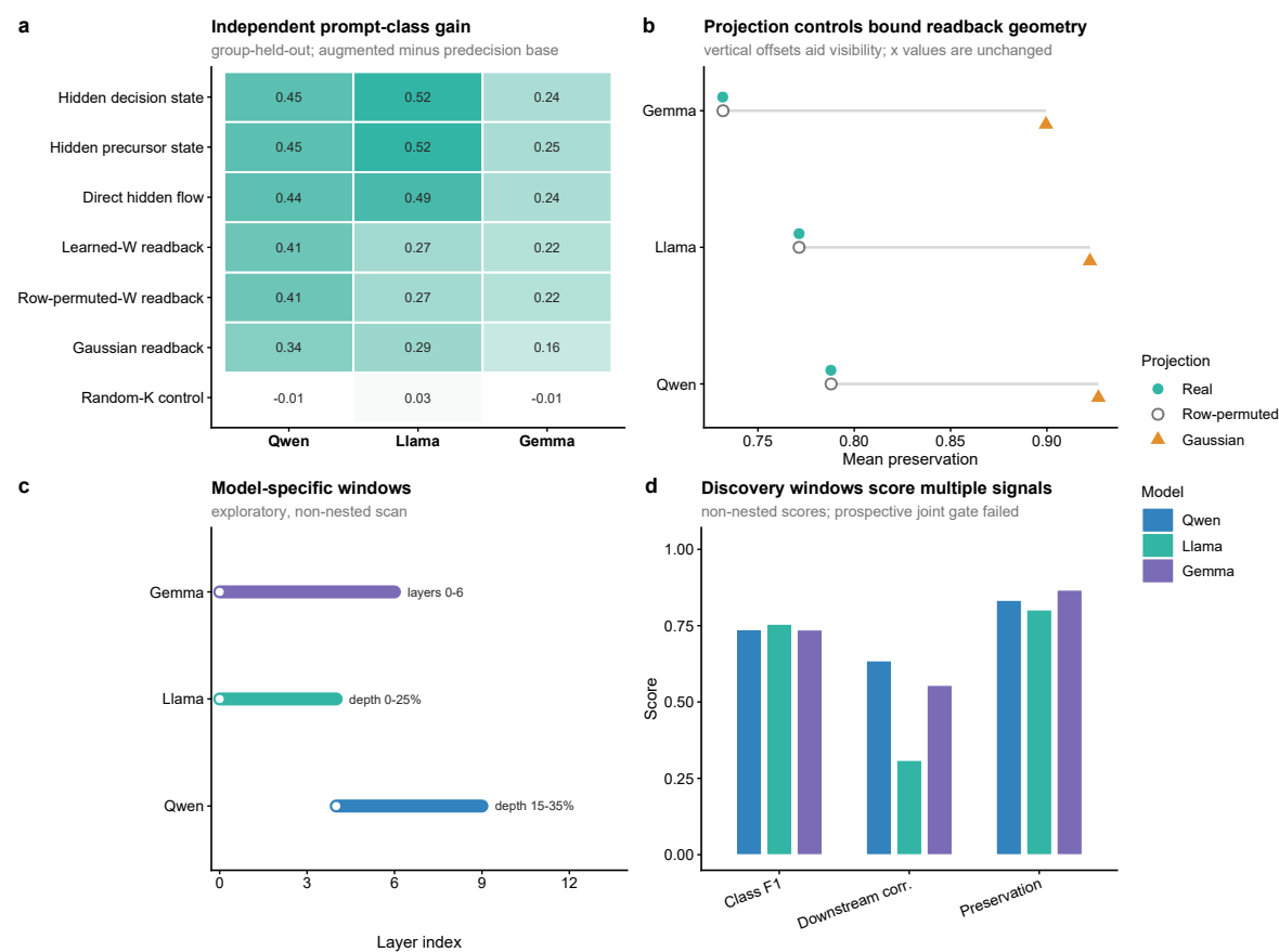
Fig. 2 | Coordinate audit and exploratory functional registration. a, Group-held-out prompt-condition-class macro-F1 gain when each proxy augments the same predecision base state. Proxy reduction was fitted within each training fold. b, Projection-selection geometry under real, row-permuted and Gaussian projection matrices. The three projection types are offset vertically within each model for visibility; their horizontal preservation values are unchanged. c, Exploratory model-specific windows. d, Discovery-scan scores for clean-relative preservation, prompt-condition-class information and downstream coupling. The stored preservation field was previously labelled topology; it is not a topology-separation test. The construction-aligned decision profile is excluded from panel a and shown only as an audit item in Extended Data Fig. 2. Readbacks remain diagnostic observables. A prospective 24-graph test failed the joint three-checkpoint window-recurrence gate (Supplementary Methods Table 2), so these data-selected windows remain exploratory. See Source Data Fig. 2 and Source Data manifest.
