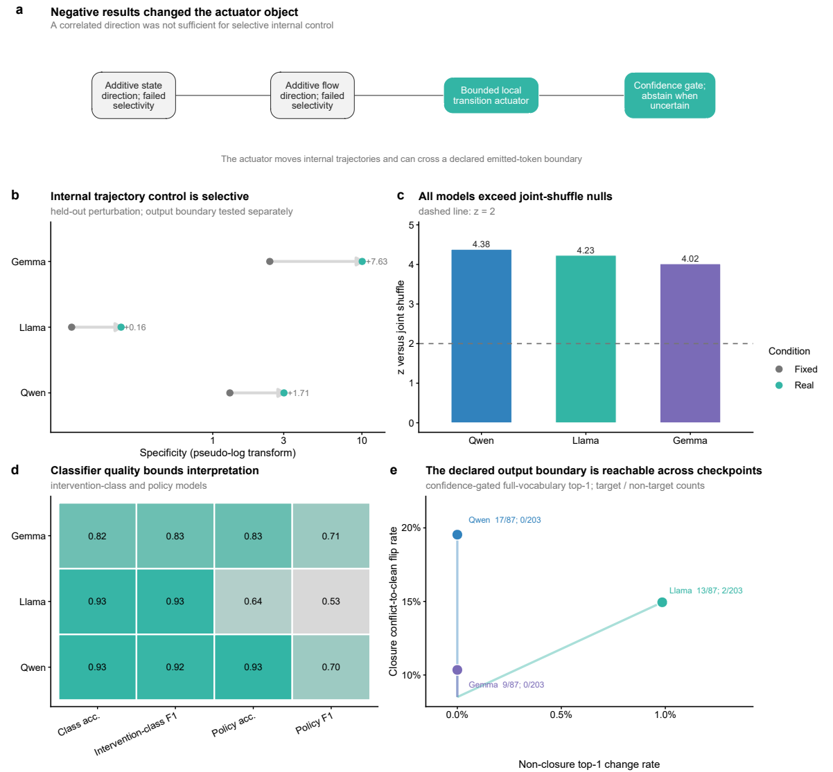
Fig. 5 | A bounded local actuator controls trajectories and a declared output boundary. a, Additive failures, bounded actuator and gate. b, Real-versus-fixed internal specificity. c, Real policy versus 50 joint-label shuffles. d, Prompt-condition and policy-classifier quality. e, Strict full-vocabulary conflict-to-clean crossings among 87 held-out closure prompts and collateral changes among 203 non-closure prompts: Qwen, 17/87 and 0/203; Llama, 13/87 and 2/203; Gemma, 9/87 and 0/203. Clean and conflict are provenance-defined candidate labels, not correct and incorrect answers; counts do not measure accuracy. See Extended Data Fig. 6f for action reassignment, Supplementary Methods Table 5 for non-crossings, and Source Data Fig. 5 and manifest.
