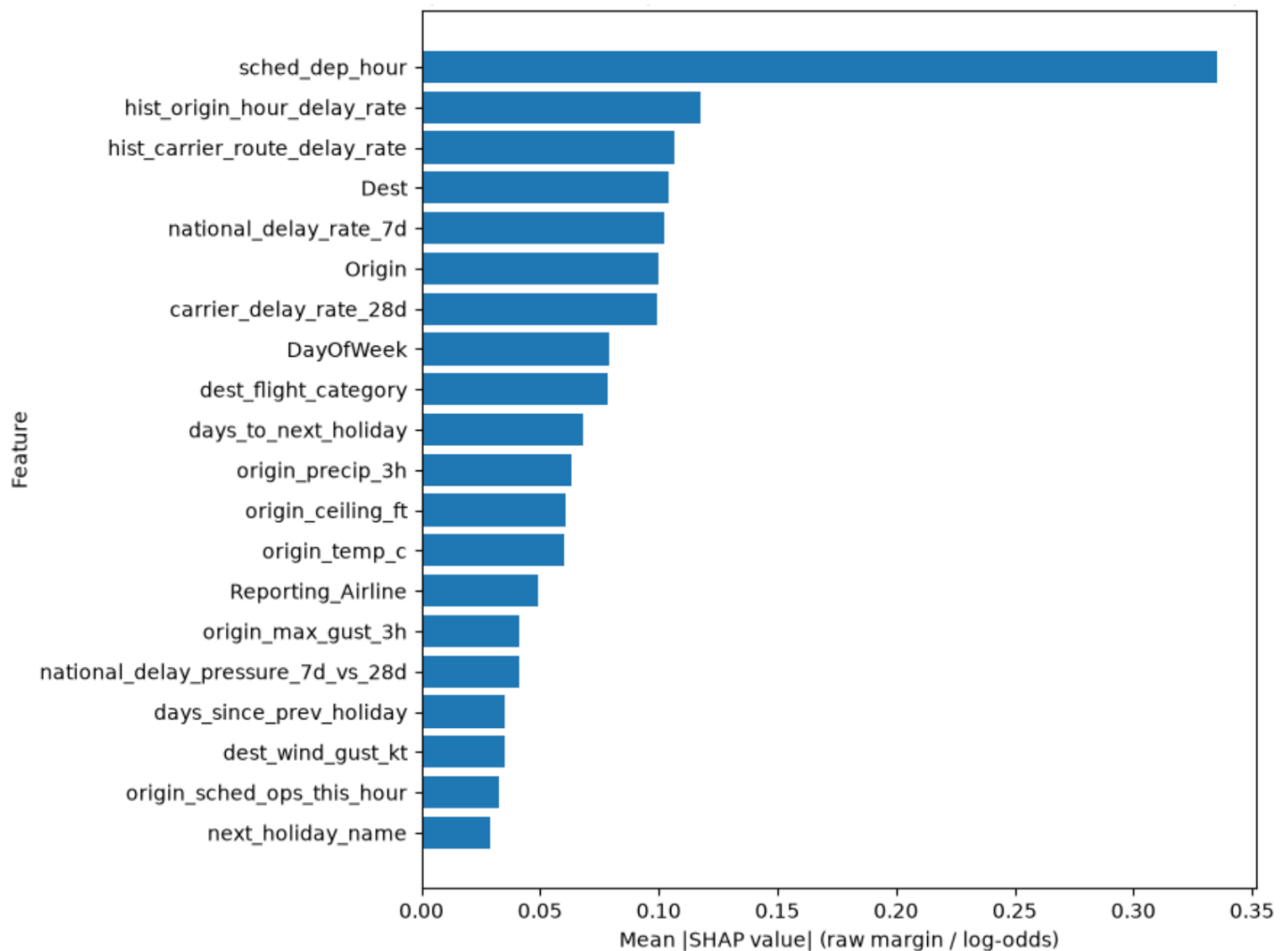
Figure 5. Experiment 3b top TreeSHAP model drivers on the 2025 validation sample.
