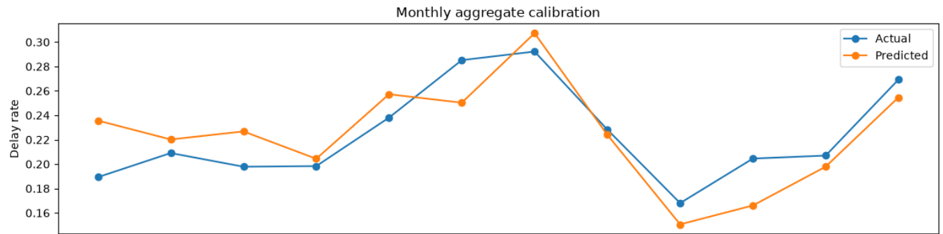
Figure 3. Experiment 3b monthly aggregate calibration on 2025 validation.
