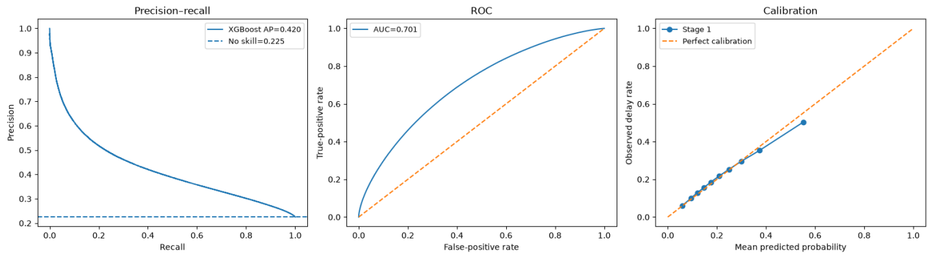
Figure 2. Experiment 3b aggregate precision-recall, ROC, and calibration curves on 2025 validation.
