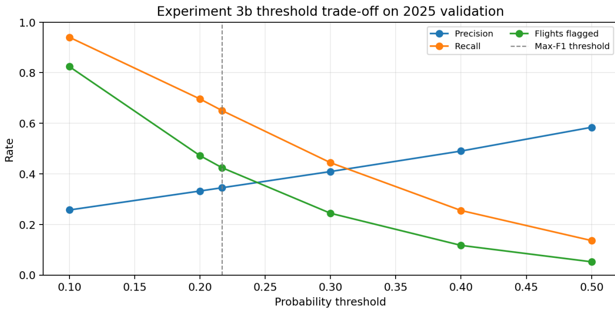
Figure 4. Precision-recall-alert-volume trade-off for Experiment 3b.
