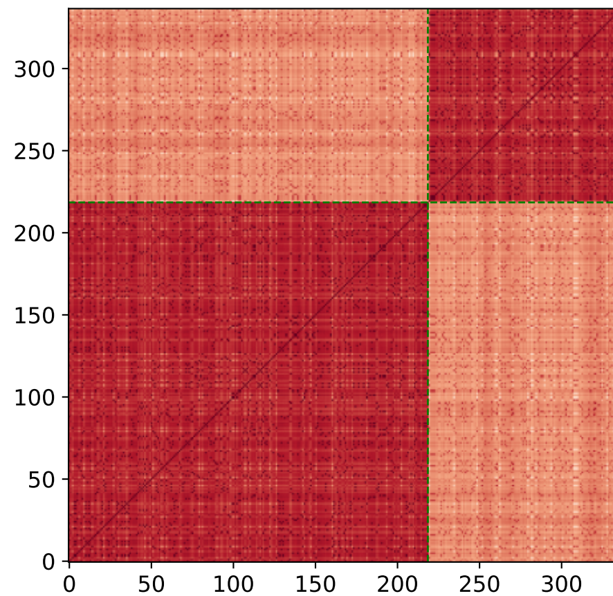
Cosine sim — GraPPI base interf_mut
