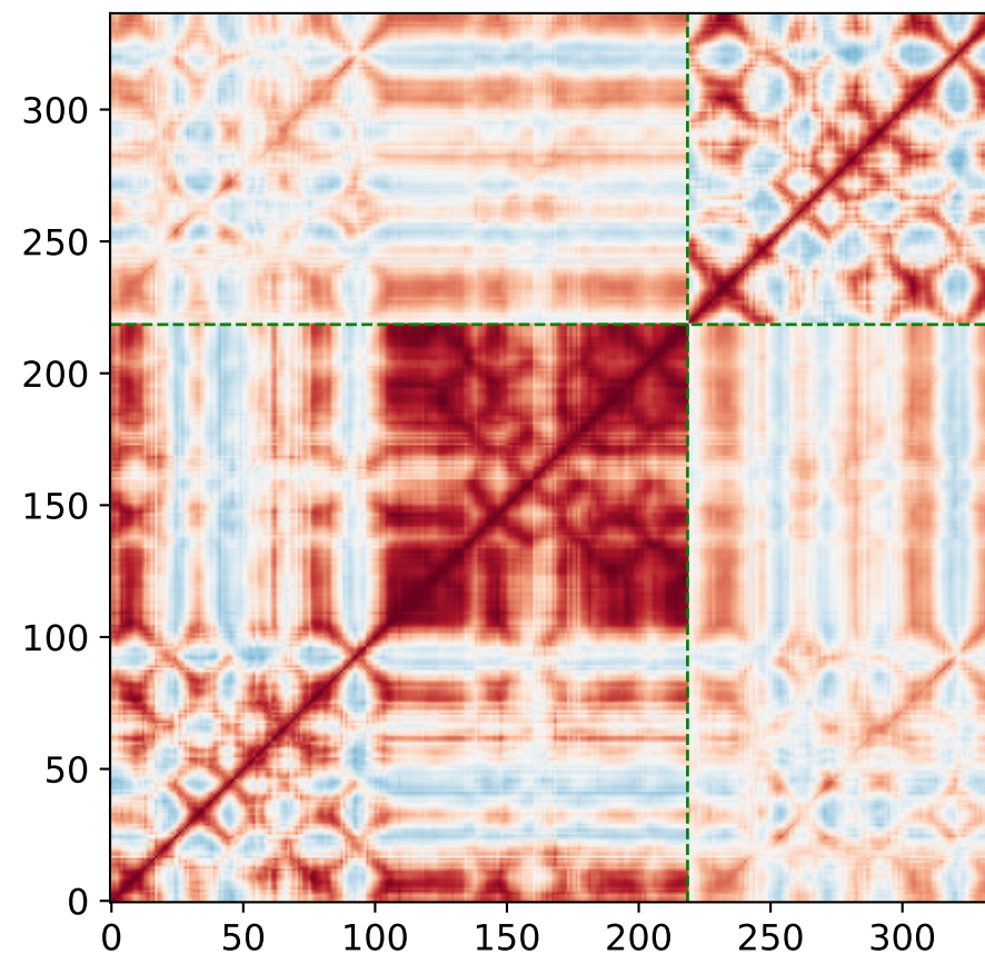
Cosine sim — untrained GraPPI base
