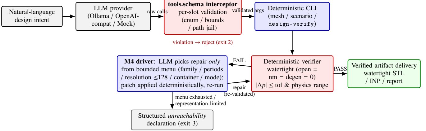
Figure 2: The agentic closed loop (v8.0). The LLM is confined to proposing schema slots: a deterministic interceptor validates every call (reject on violation) before execution, the verification ladder is purely deterministic, and repair decisions are re-validated from a bounded strategy menu — yielding either a verified watertight artifact or a structured unreachable declaration, never a silently degraded mesh.
