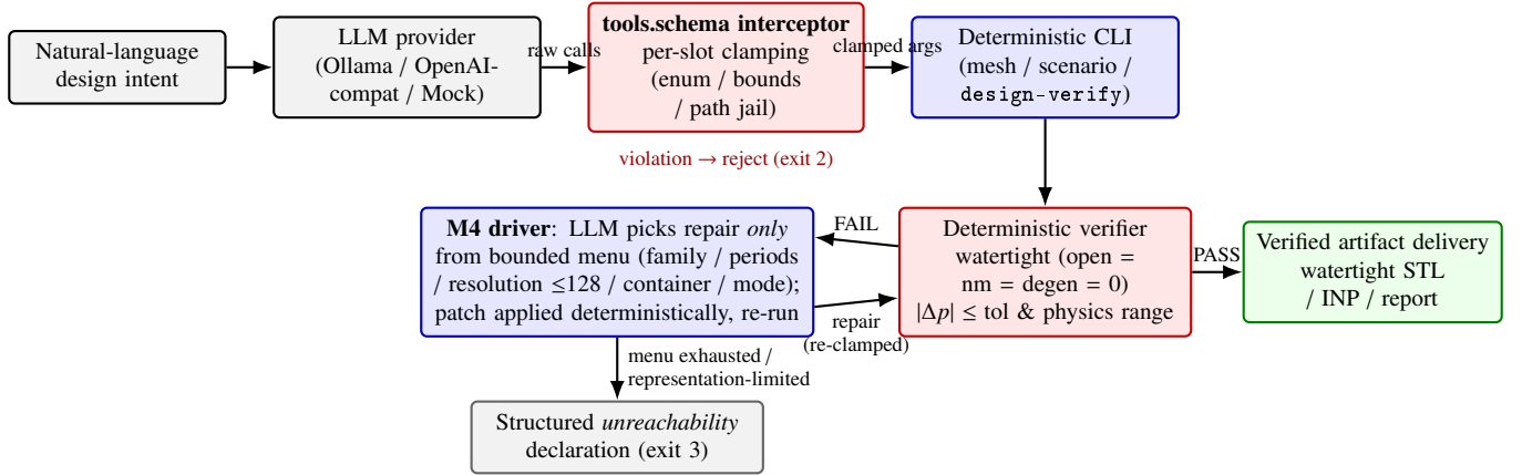
Figure 1: The agentic closed loop (v8.0). The LLM is confined to proposing schema slots: a deterministic interceptor clamps or rejects every call before execution, the verification ladder is purely deterministic, and repair decisions are re-clamped from a bounded strategy menu — yielding either a verified watertight artifact or a structured unreachable declaration, never a silently degraded mesh.
