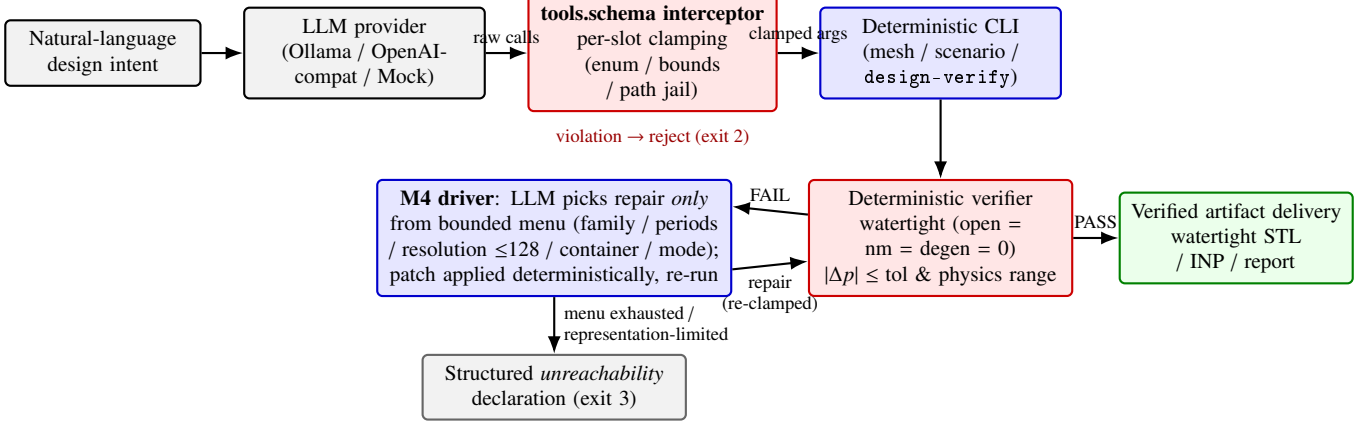
Figure 2: The agentic closed loop (v8.0). The LLM is confined to proposing schema slots: a deterministic interceptor clamps or rejects every call before execution, the verification ladder is purely deterministic, and repair decisions are re-clamped from a bounded strategy menu — yielding either a verified watertight artifact or a structured unreachability declaration, never a silently degraded mesh.
