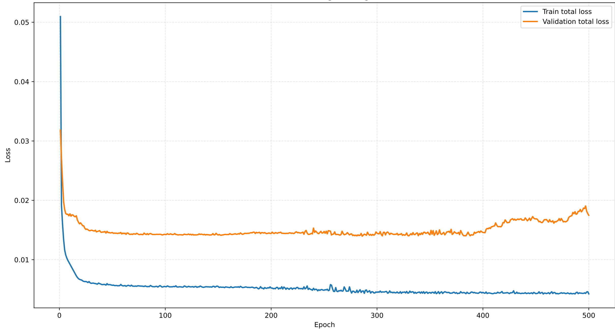
DSCGNet Training Convergence
