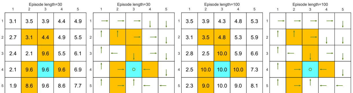
(g) Final value and policy with episode length=30
