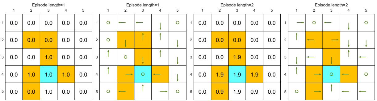
(a) Final value and policy with episode length=1
